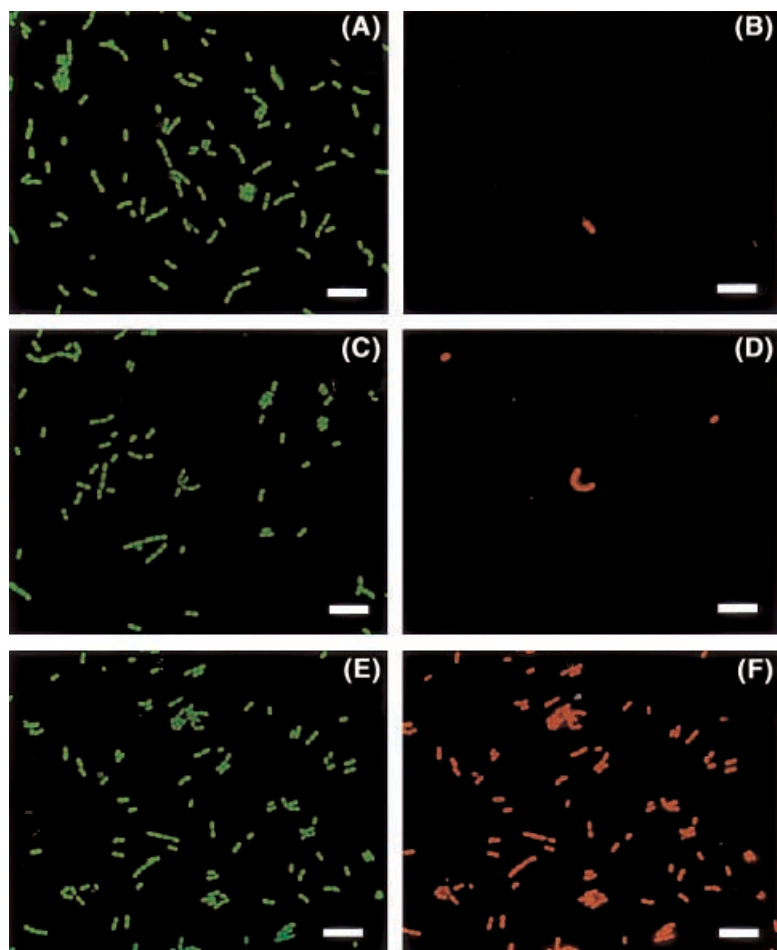
Fig. 4. Fluorescence microscopic observation of S. mutans exposed to ozonated water. After exposure to ozonated water (4 mg/l) for 120 s, bacterial cells were stained with LIVE/DEAD ® BacLight ™ Bacterial Viability Kit solution and observed with a fluorescence microscope (BX-50; Olympus Optical Co., Ltd., Tokyo, Japan). After S. mutans was exposed with medium (A, B), distilled water (C, D) or ozonated water (E, F), both viable and nonviable cells exhibited fluorescent green while nonviable cells exhibited fluorescent red. Scale bar = 5 \mu m.
